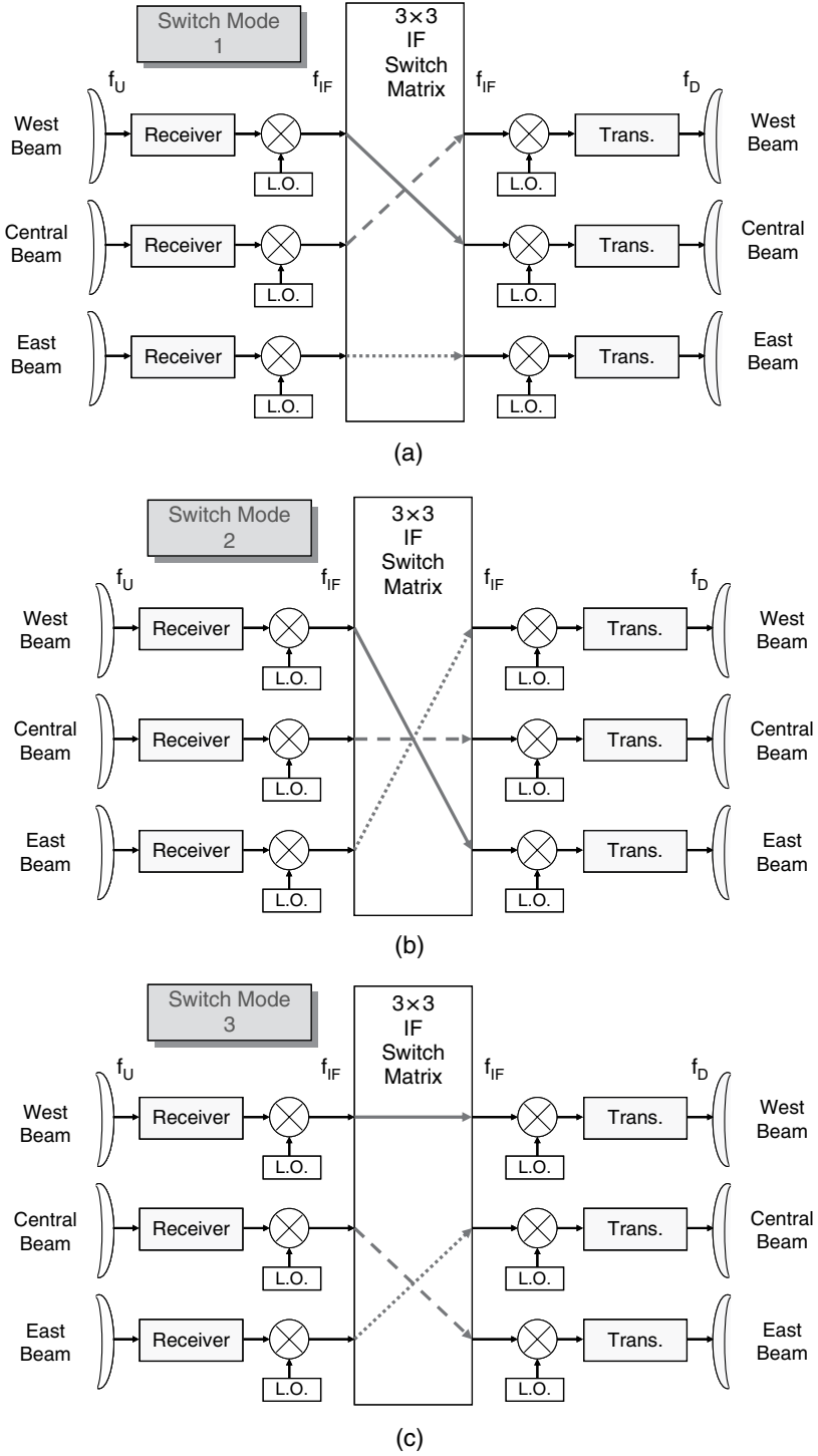
Figure 10.6 Switch matrix settings for 3 × 3 SS/TDMA network
