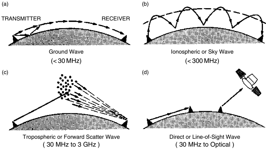
Figure 6.2 Radiowave propagation modes (source: Ippolito [1]; reproduced by permission of © 1986 Van Nostrand Reinhold)
