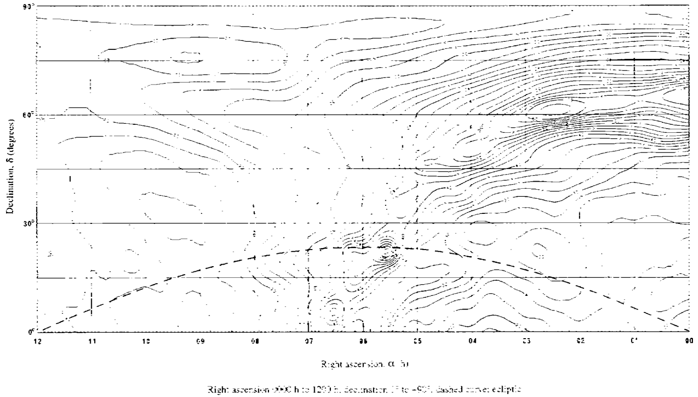
Figure 6.29 Radio sky temperature at 408 MHz (source: ITU-R [23]; reproduced by permission of International Telecommunications Union)
