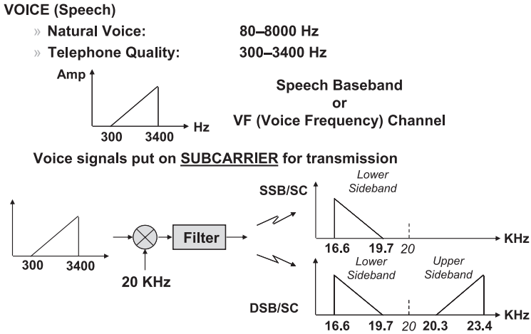
Figure A.2 Analog voice baseband formats
