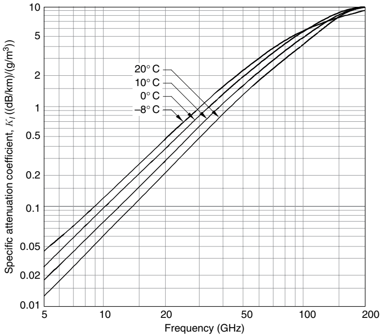
Figure 6.13 Specific attenuation for clouds as a function of frequency and temperature ( source: ITU-R [10]; reproduced by permission of International Telecommunications Union )
