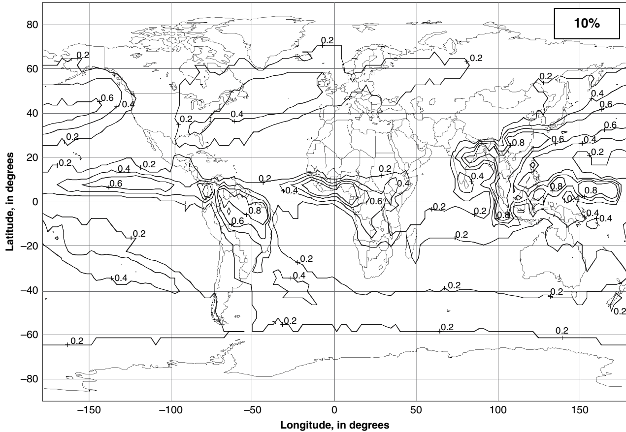
Figure 7.6 Normalized total columnar content of cloud liquid water exceeded for 10 % of the year, in \text{kg/m}^2 (source: ITU-R P.840-3 [10]; reproduced by permission of International Telecommunications Union)
