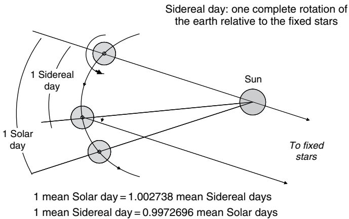
Figure 2.6 Sidereal time
