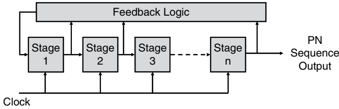
Figure 10.8 n-stage feedback shift register PN sequence generator
