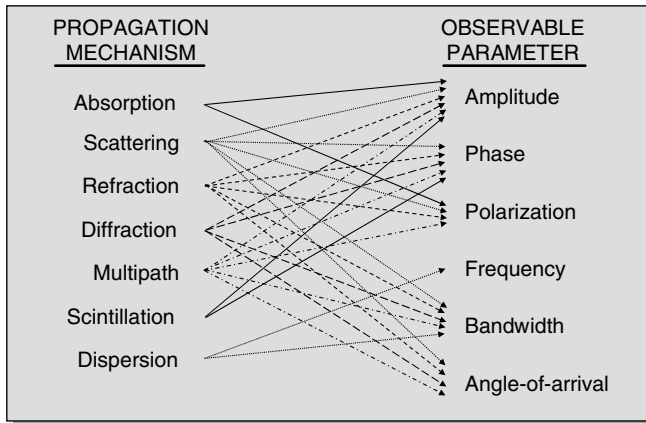
Figure 6.3 Radiowave propagation mechanisms and their impact on the parameters of a communications signal (based on Ippolito [1], Fig 2.5; reproduced by permission of © 1986 Van Nostrand Reinhold)
